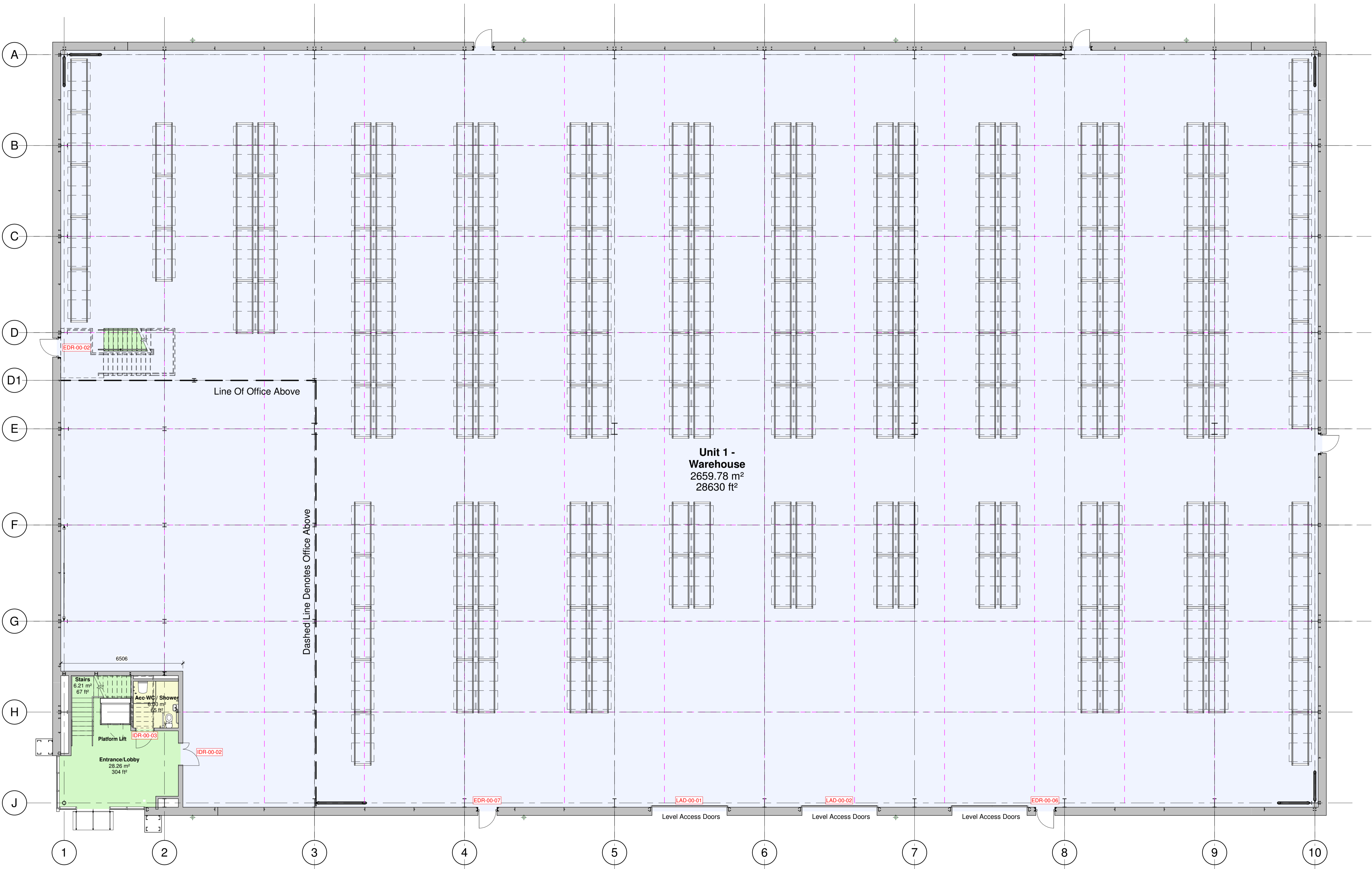
20-00- Racking Option 2-Level 00 1:100
