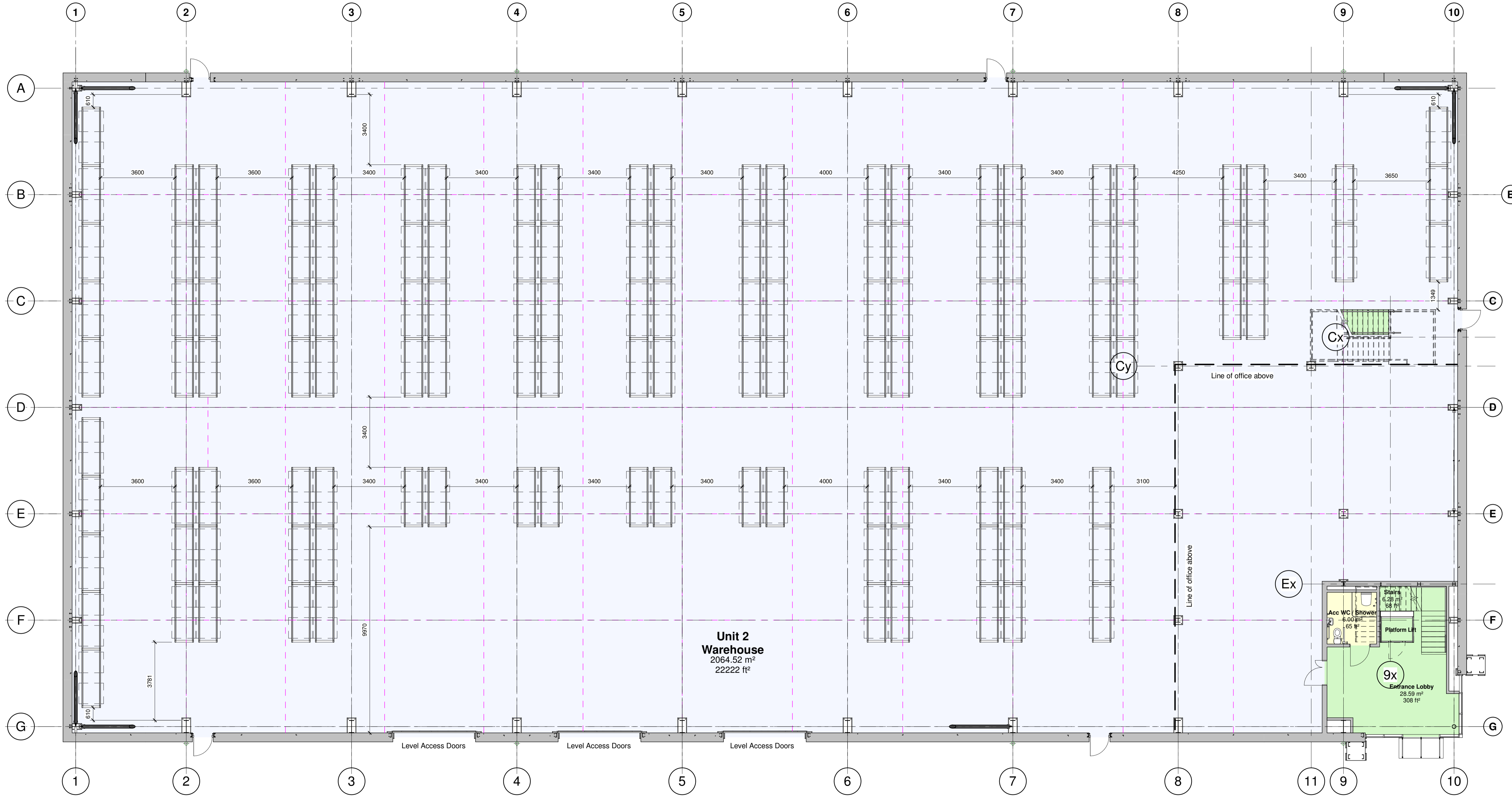
20-00 Unit 2 Racking Option 2 1:100
