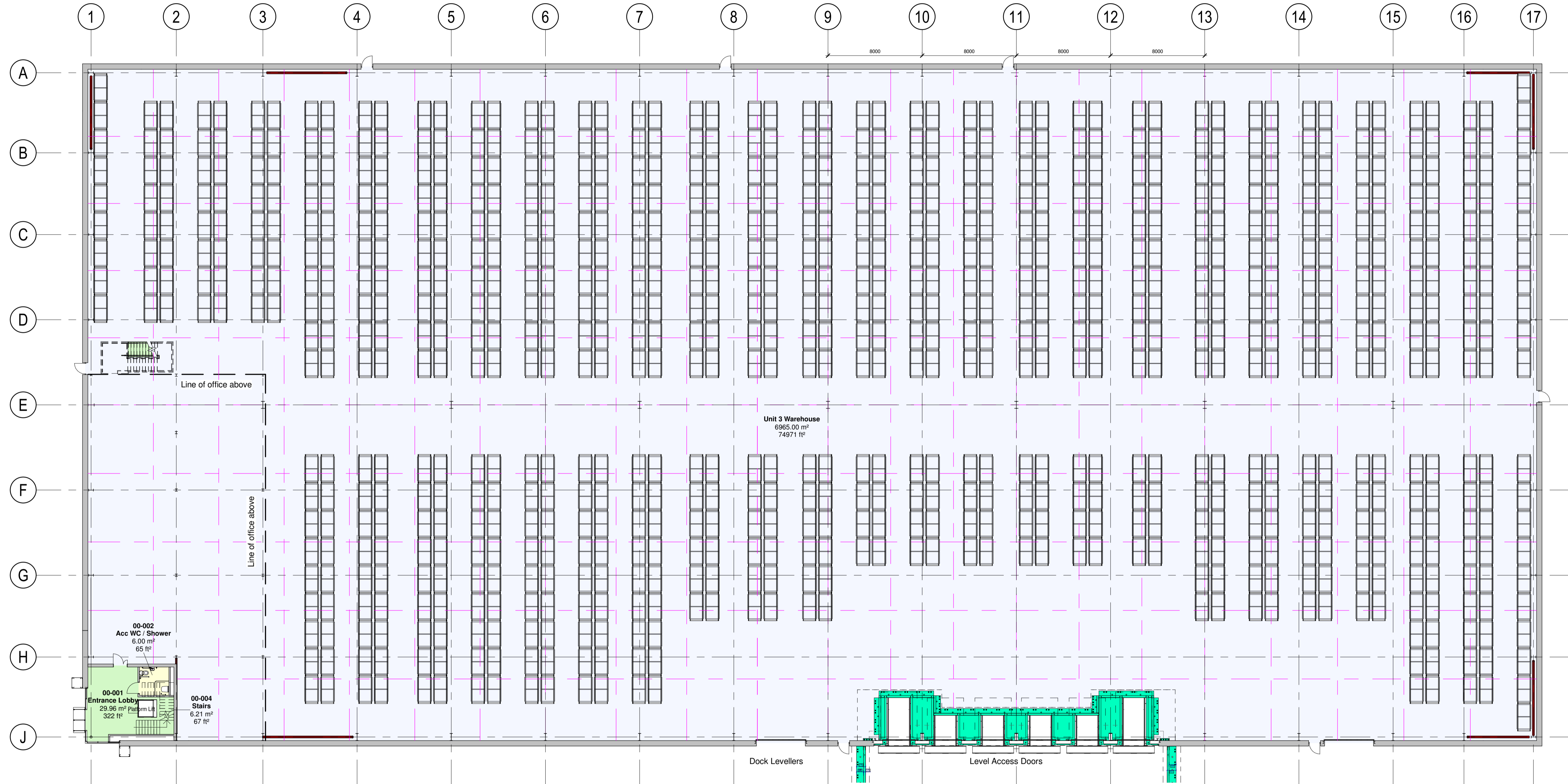
20-00- Racking Option 1 - Level 00 1 : 200
