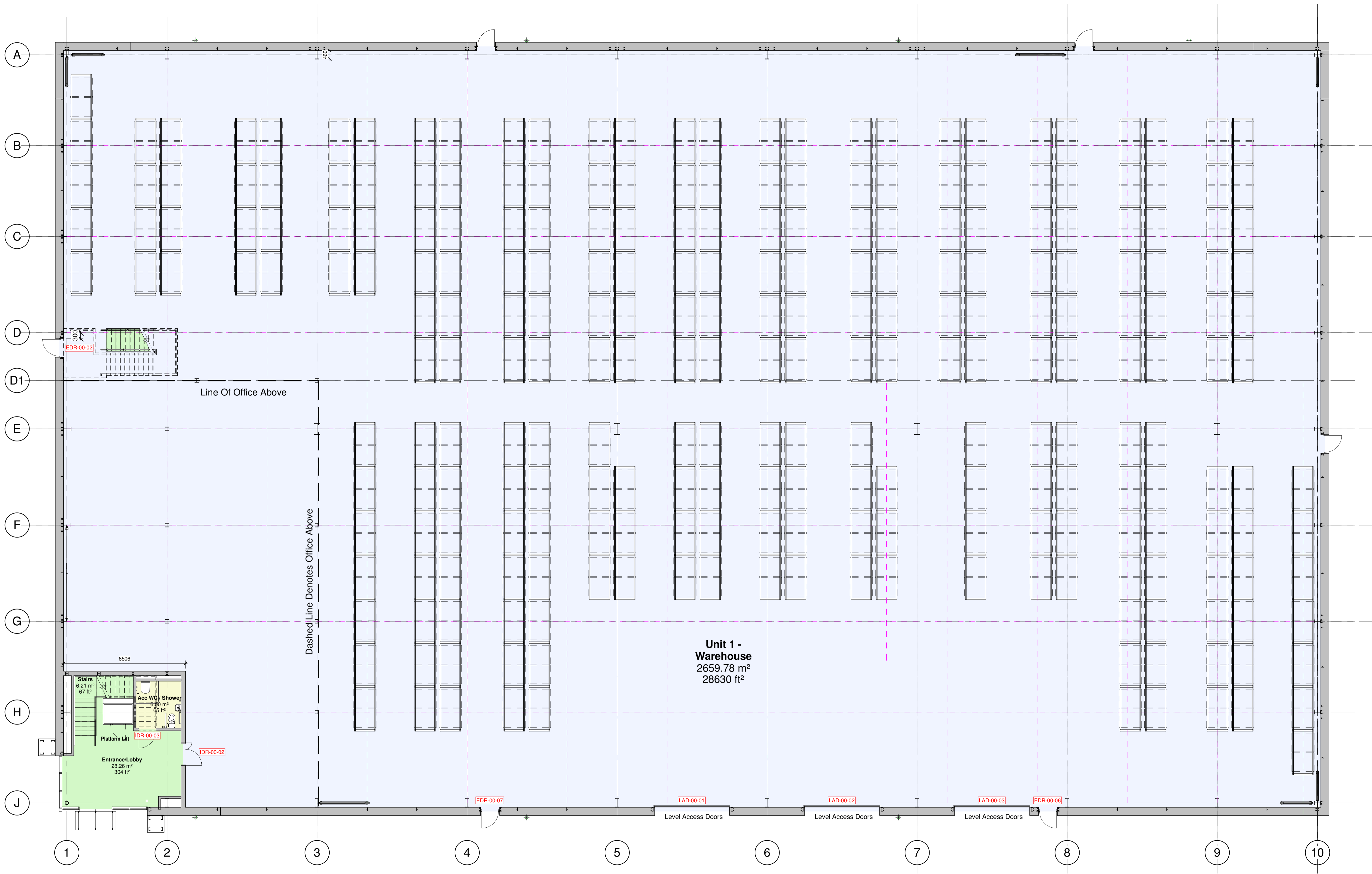
1 20-00- Racking Option 1-Level 00 1:100
