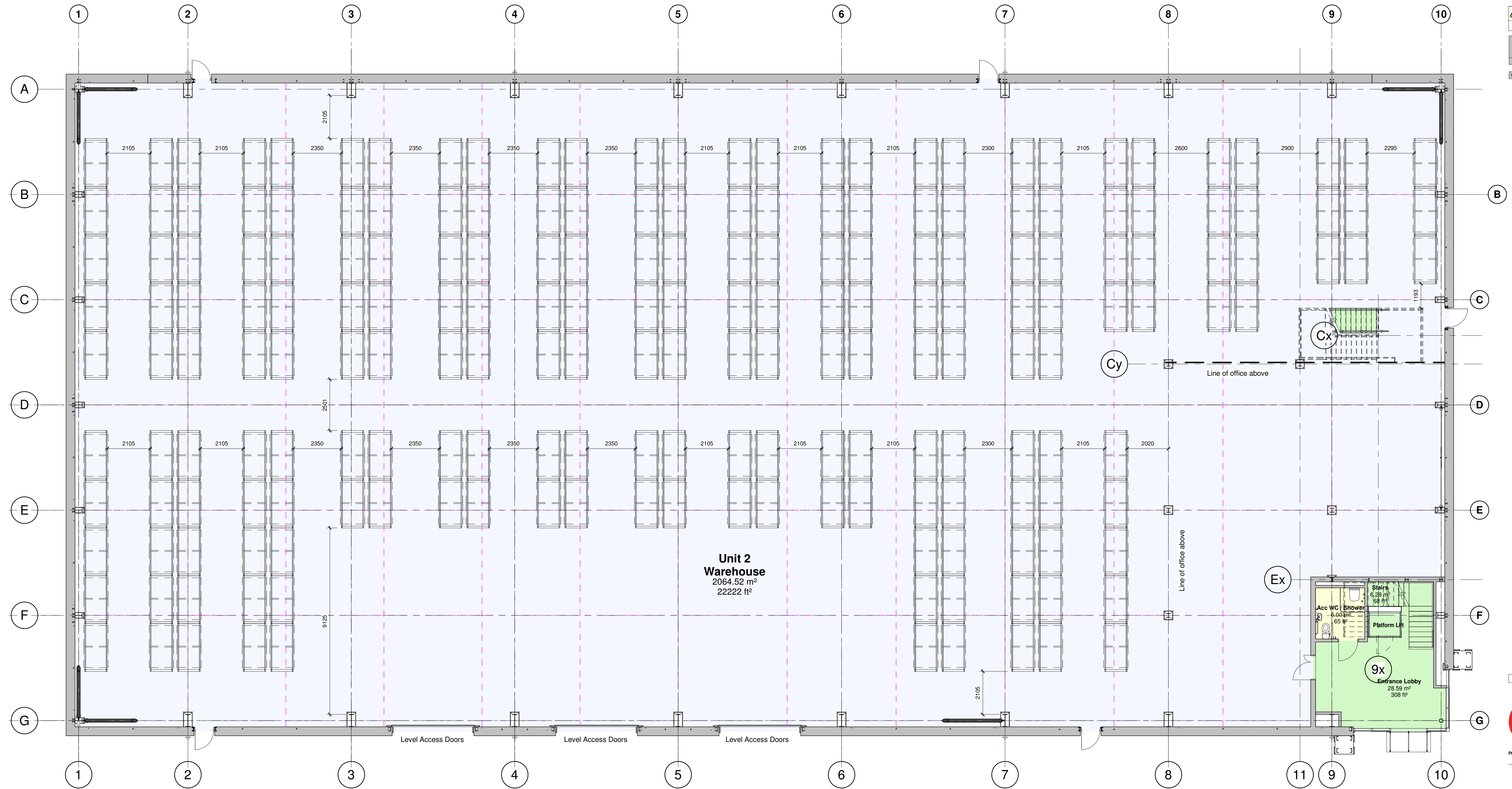
20-00 Unit 2 Racking Option 1 1:100
